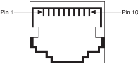
Figure 4. 10-Position Modular Jack Pin Locations
