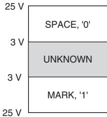
Figure 8. RS-232 Signals
