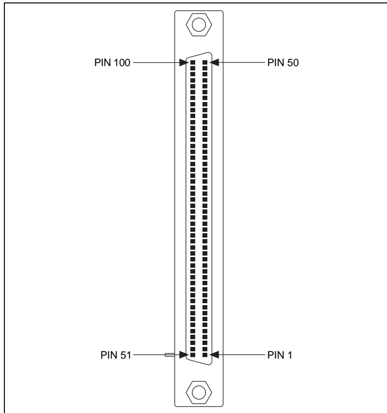
Figure 2-10. 100-Pin Connector Pin Locations
