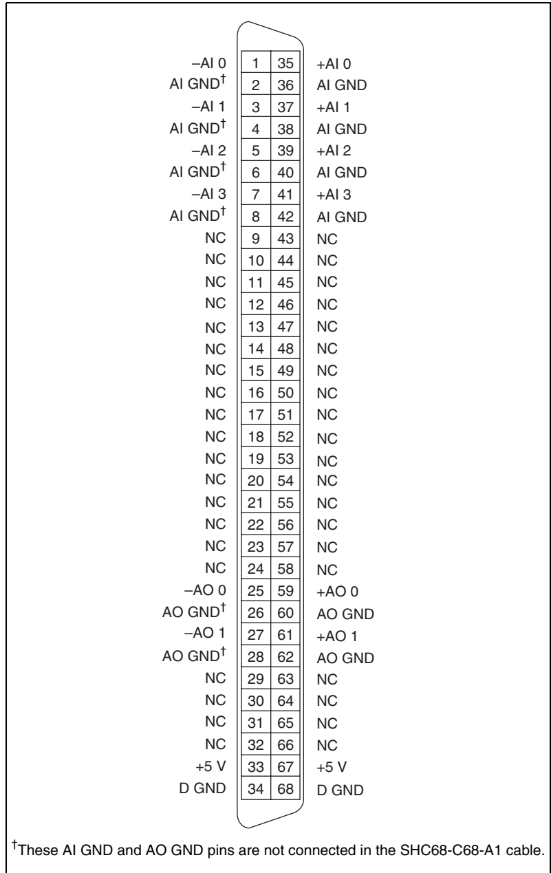
Figure 3-1. BNC-2140 External 68-Pin Analog Connector
