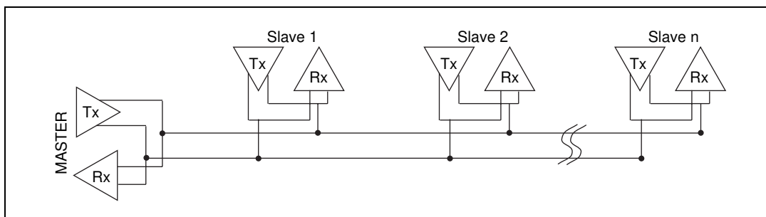
Figure A-2. Typical Half-Duplex System
