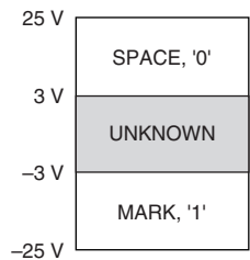
Figure 7. RS-232 Signals
