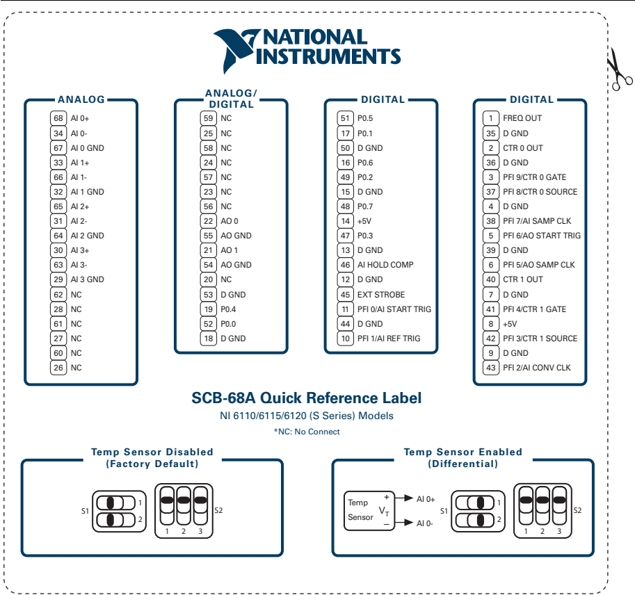
Figure 1. NI 6110/6115/6120
