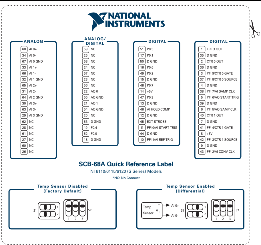
Figure 1. NI 6110/6115/6120
