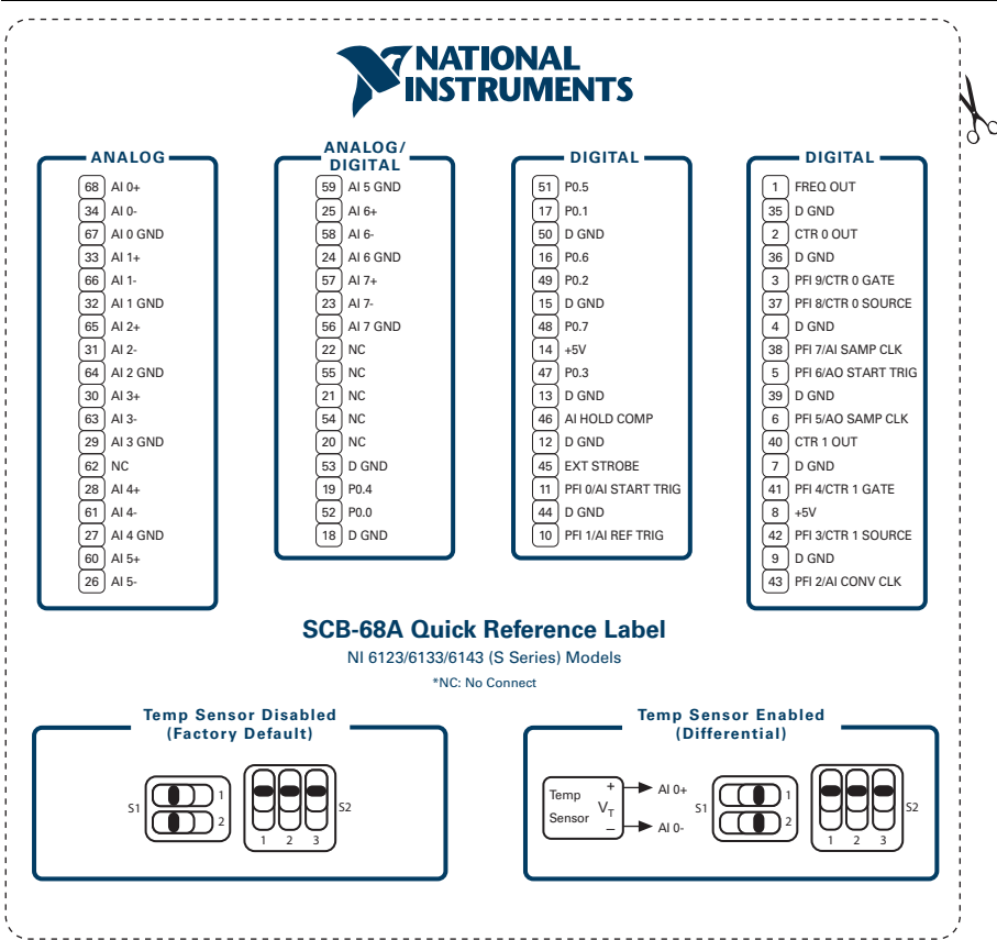
Figure 4. NI 6123/6133/6143
