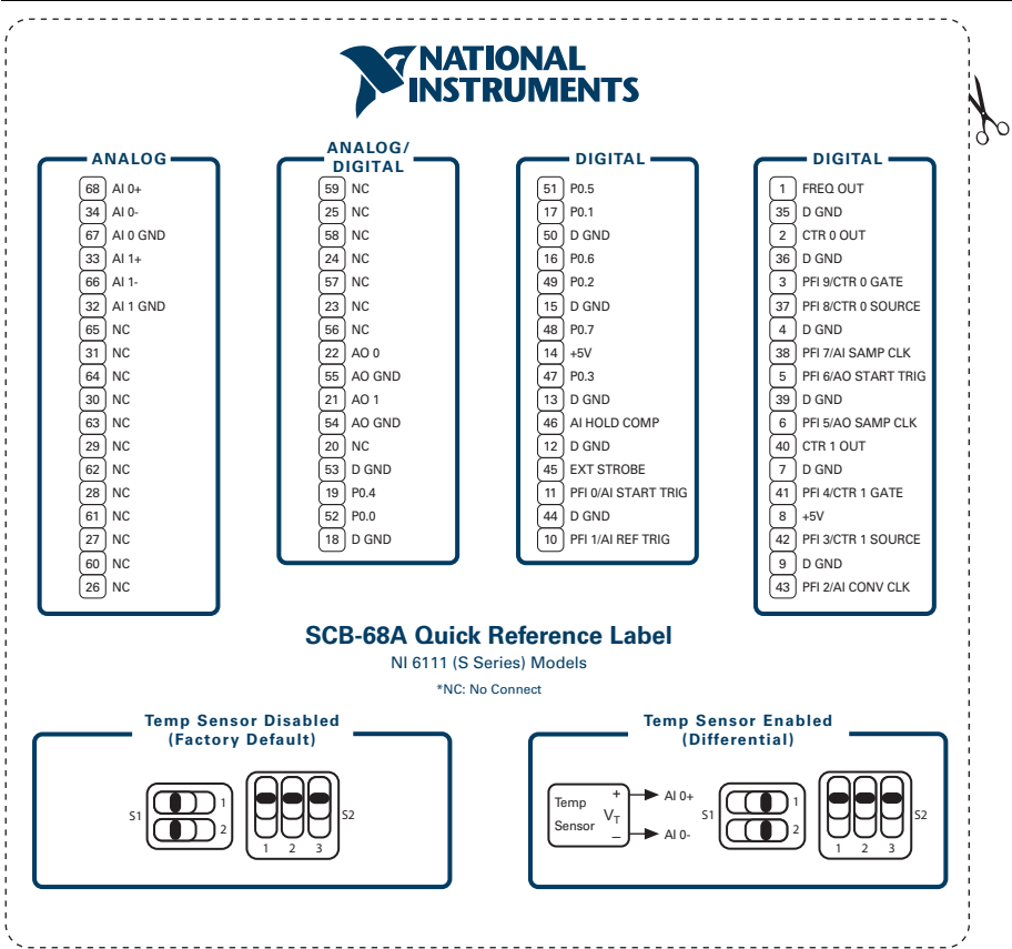
Figure 2. NI 6111
