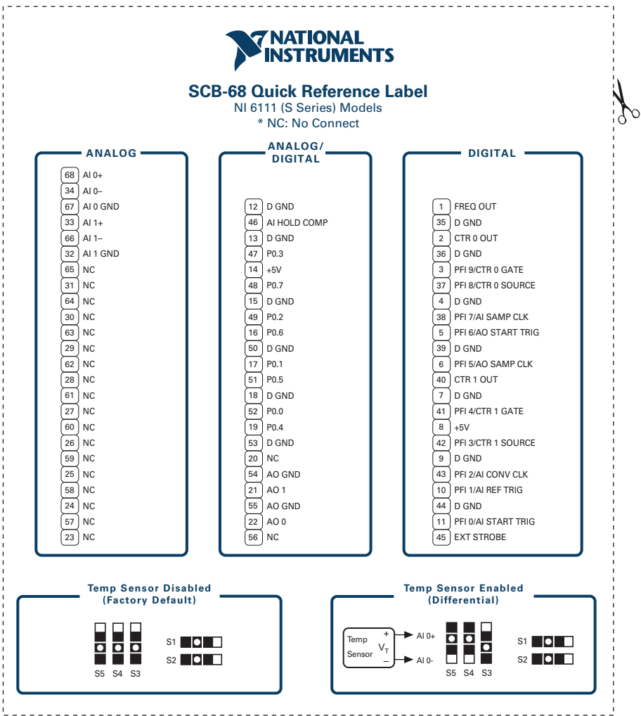
Figure 2. NI 6111
