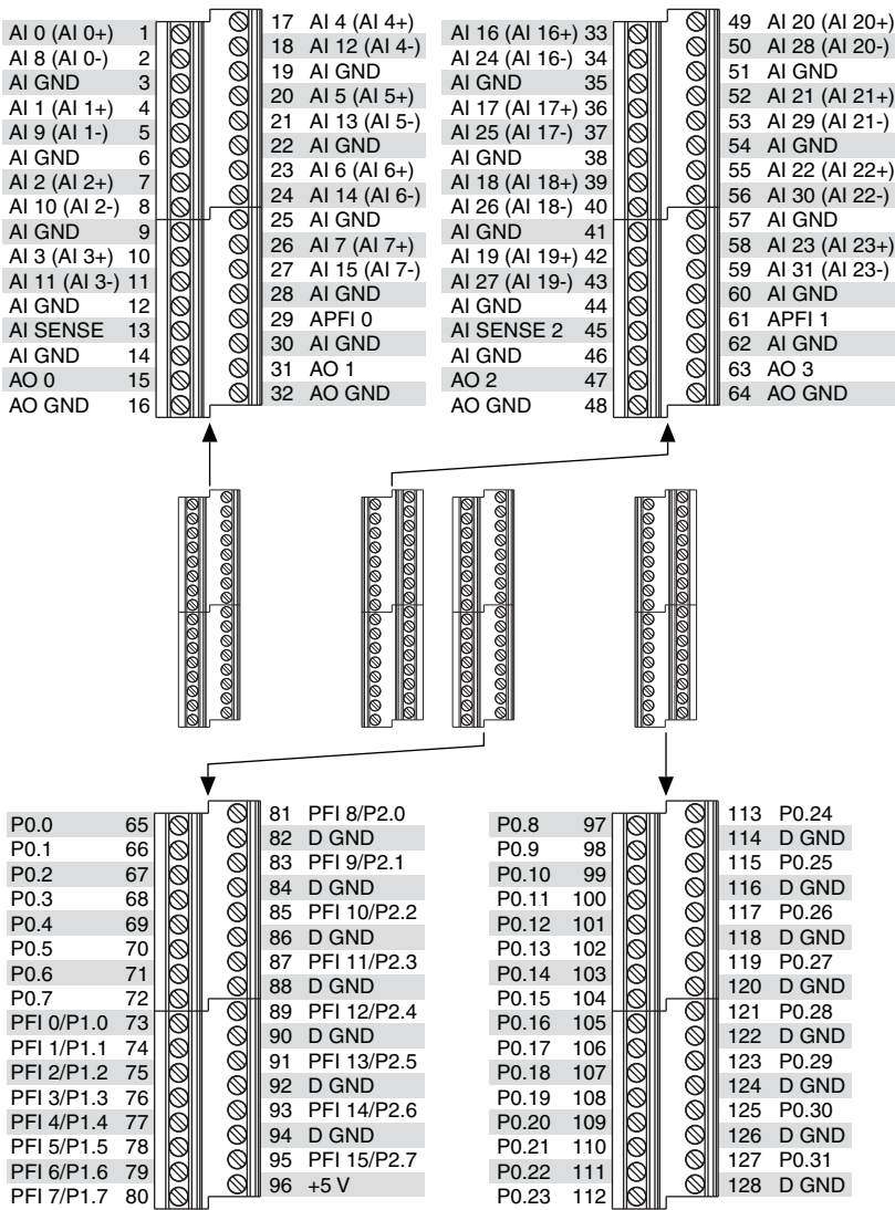
Figure A-32. USB-6289 Screw Terminal Pinout
