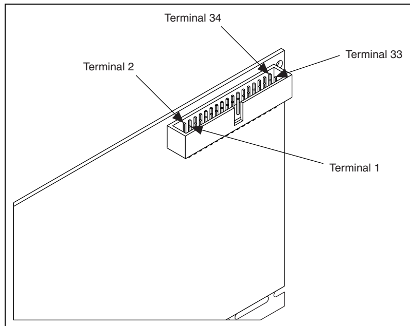
Figure 10-2. NI 6238/6239 RTSI Pinout
