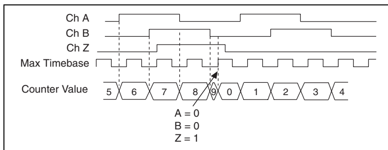
Figure 7-18. Channel Z Reload with X4 Decoding
