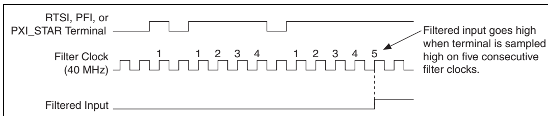
Figure 8-4. Filter Example
