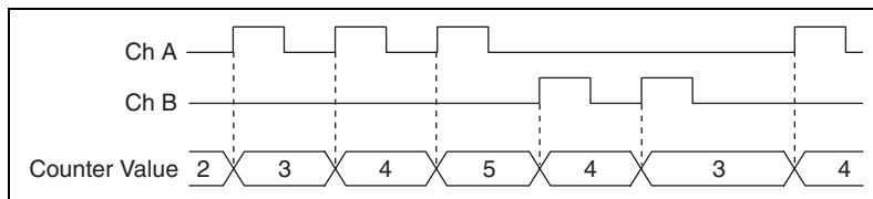
Figure 7-19. Measurements Using Two Pulse Encoders
