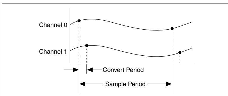
Figure 4-8. Interval Sampling
