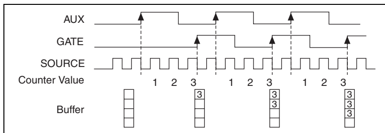
Figure 7-21. Buffered Two-Signal Edge-Separation Measurement
