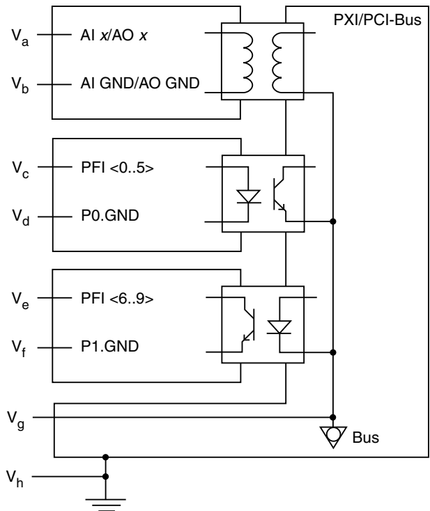
Figure 5. NI 6238 Maximum Working Voltage
