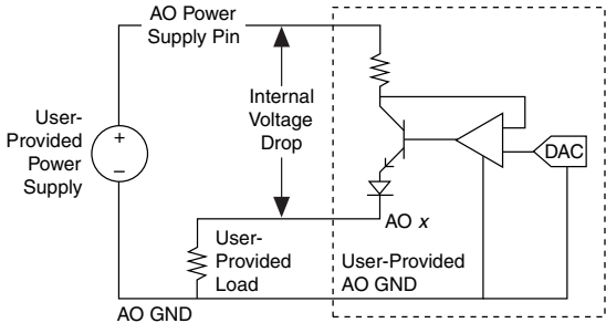
Figure 3. Analog Output
