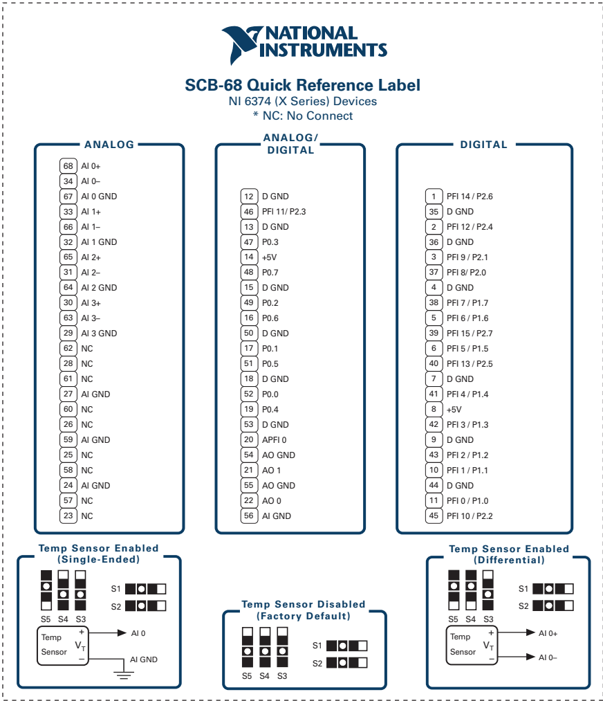
Figure 5. NI 6374 Connector 0
