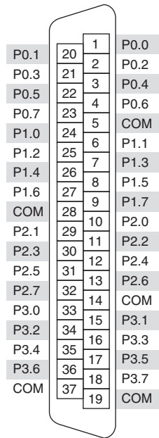
Figure 3-1. NI 6510 Pin Assignments
