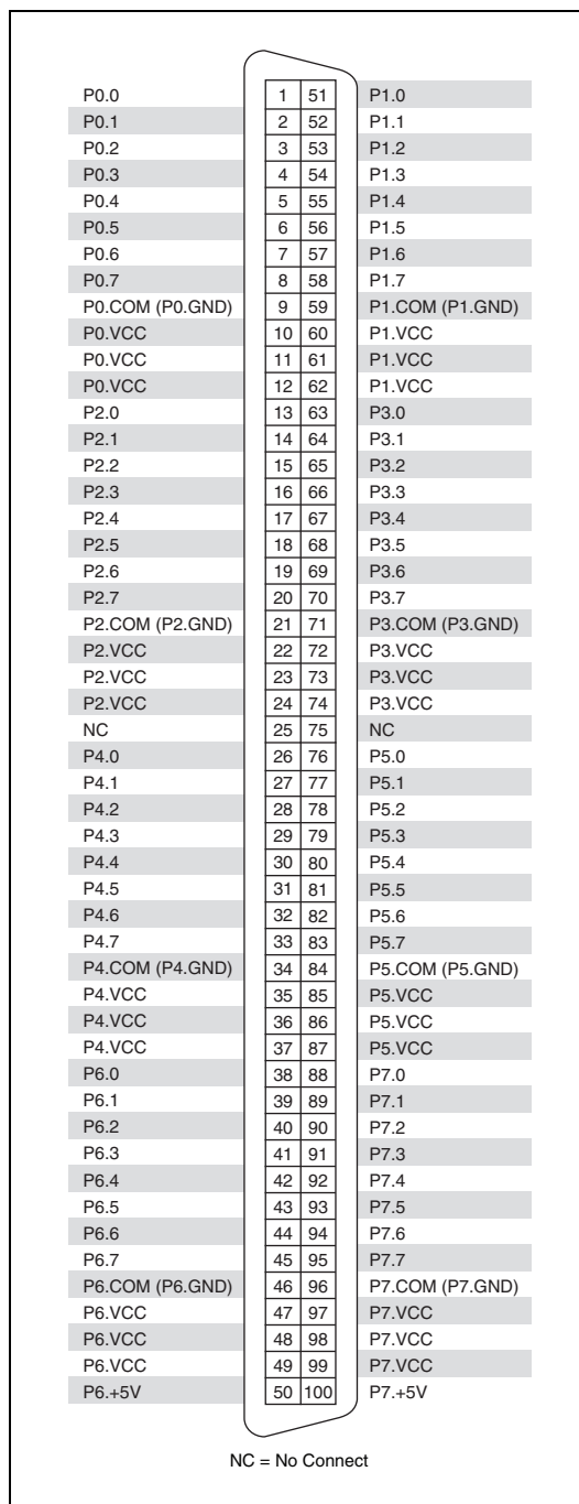
Figure 4. NI 6512 Pin Assignments for the SH100-100-F Cable
