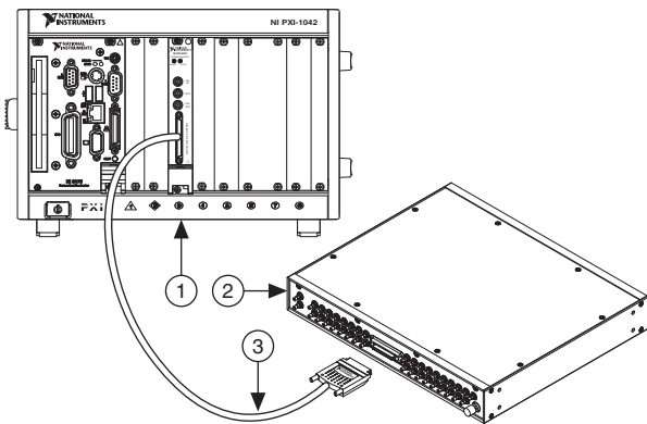
Figure 8. Connecting the NI SMB-2163 Accessory
