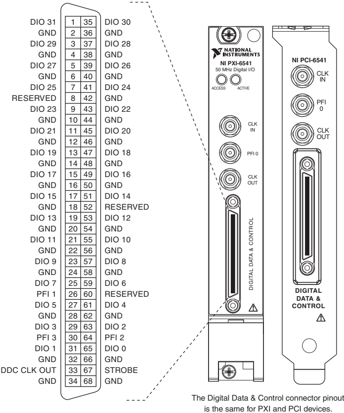
Figure 14. NI 654x Front Panel Connectors
