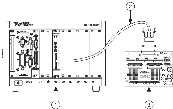
Figure 7. Connecting the NI CB-2162 Accessory
