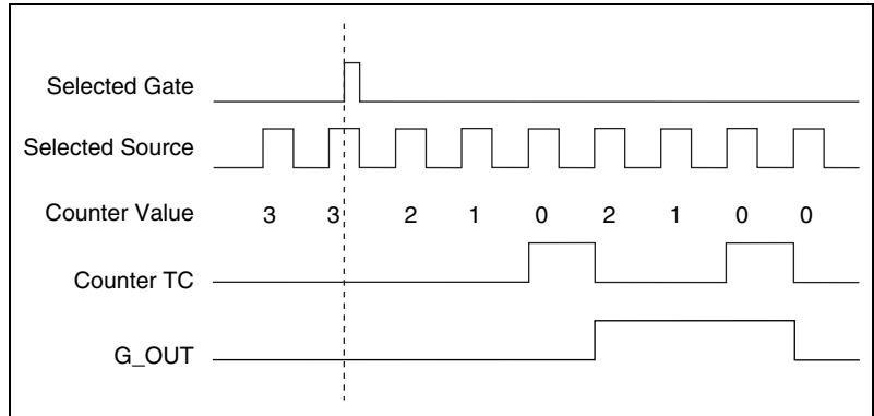
Figure 2-12. Single Triggered Pulse Generation
