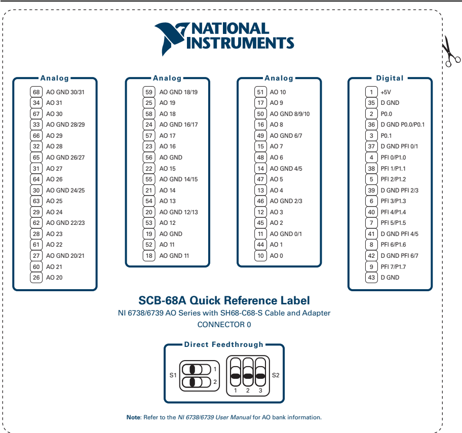
Figure 8. NI 6738/6739 Connector 0 with SH68-C68-S Cable and NI PXIe-6738/6739 Adapter
