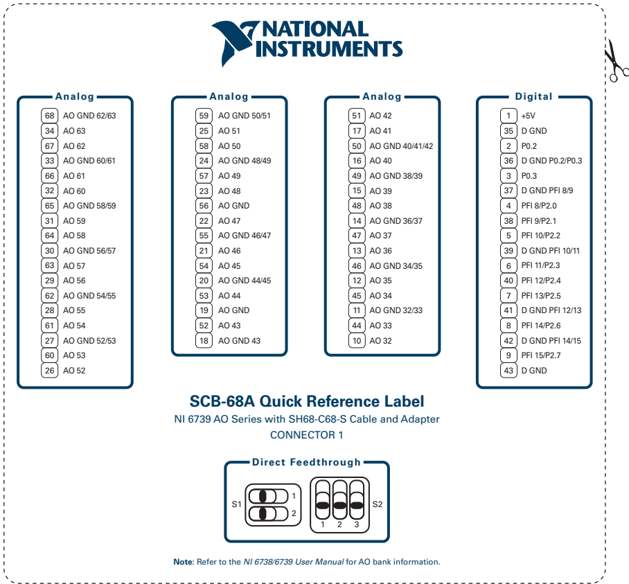
Figure 9. NI 6739 Connector 1 with SH68-C68-S Cable and NI PXIe-6739 Adapter
