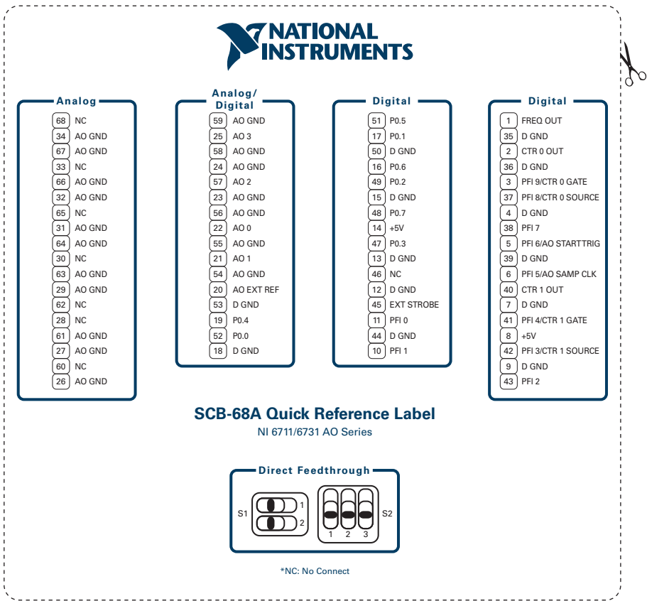
Figure 3. NI 6711/6731
