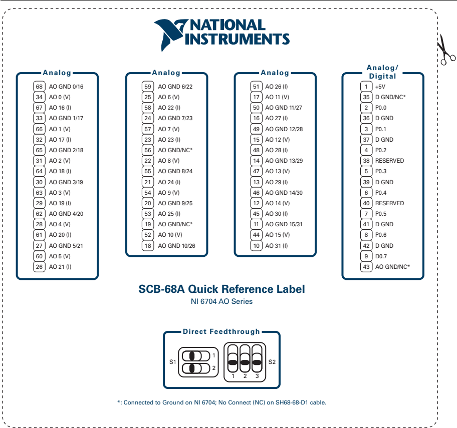
Figure 2. NI 6704
