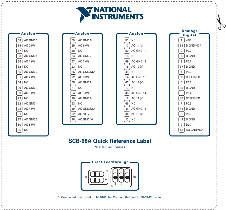
Figure 1. NI 6703
