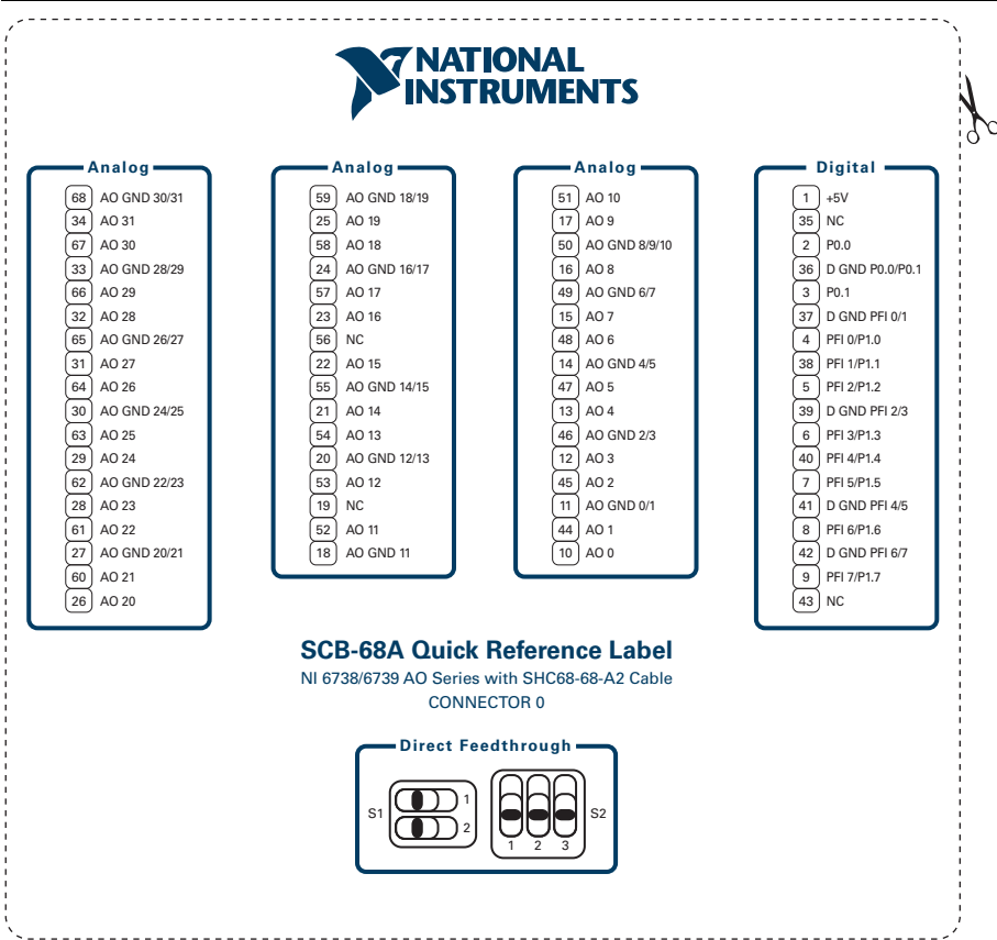
Figure 6. NI 6738/6739 Connector 0 with SHC68-68-A2 Cable
