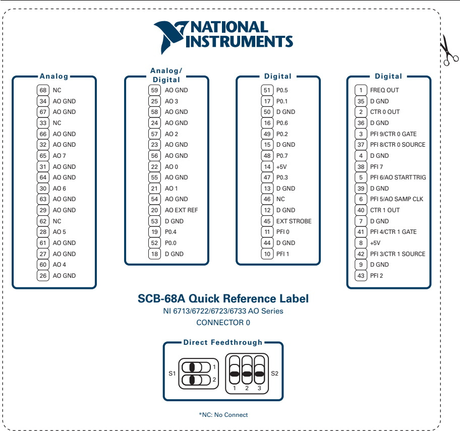
Figure 4. NI 6713/6722/6723/6733 Connector 0
