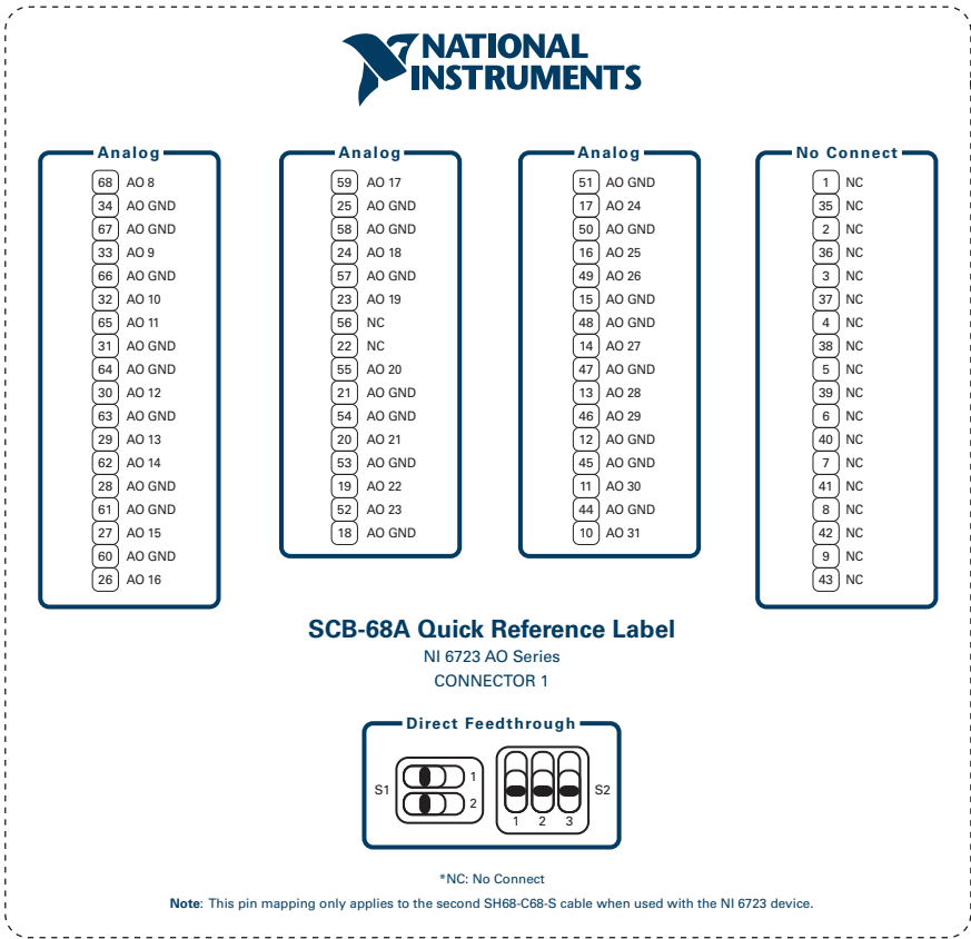
Figure 5. NI 6723 Connector 1
