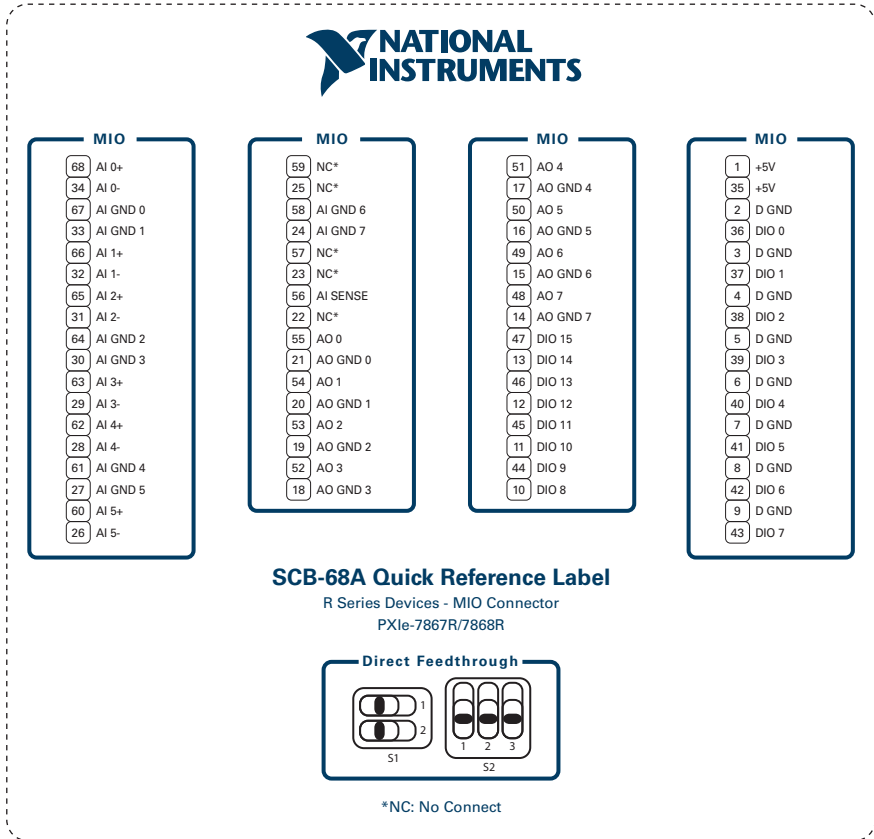
Figure 1. MIO Connector for NI PXIe-7867R/7868R
