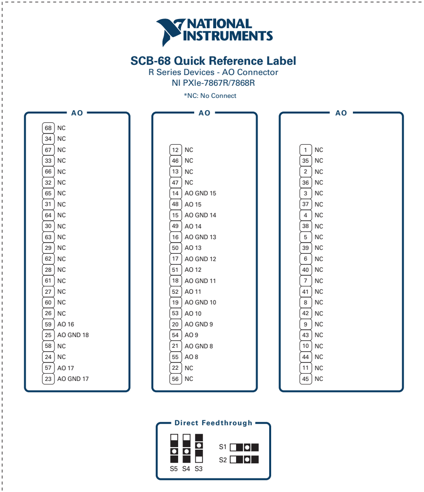
Figure 2. RAO Connector for NI PXIe-7867R/7868R
