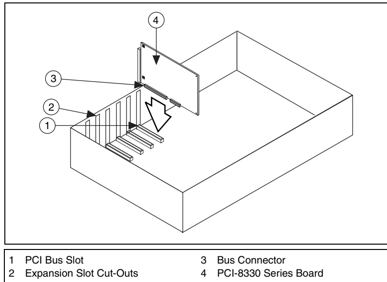
Figure 2-2. Installing the PCI-8330 Series Interface Board
