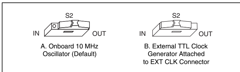
Figure C-4. CLK10 Signal Routing
