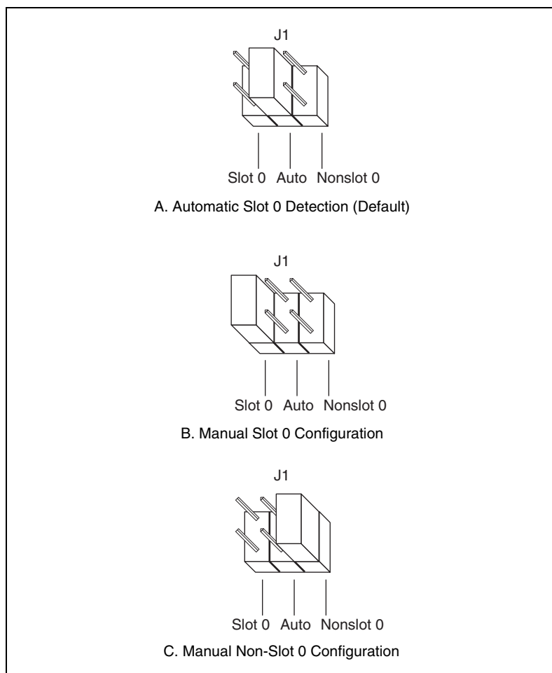
Figure C-2. VXIbus Slot Configuration
