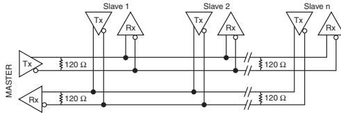
4-Wire Full-Duplex Multidrop Network Using Terminating Resistors
