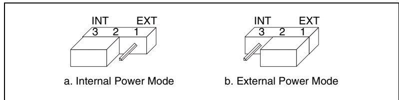
Figure E-5. Power Source Jumpers
