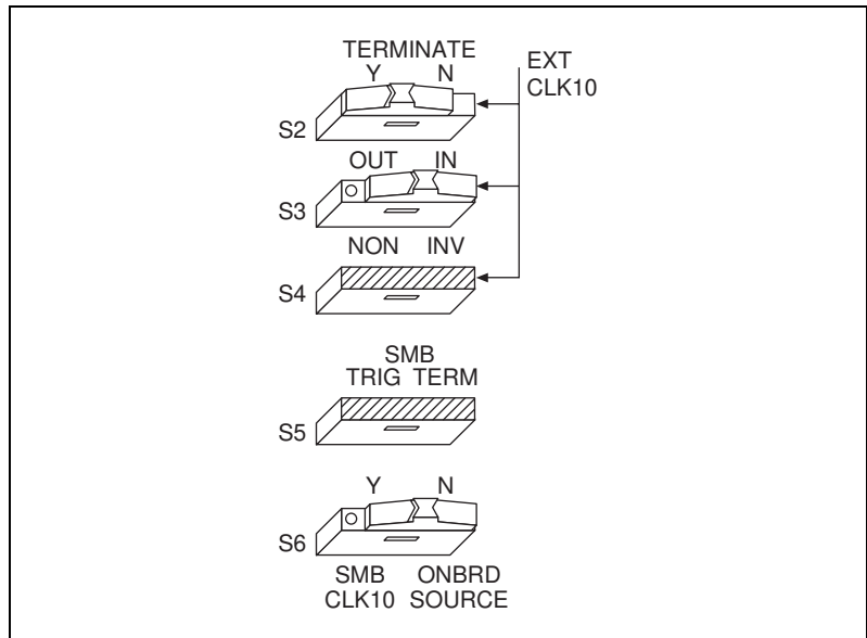
Figure C-5. Receive External CLK SMB with 50 \Omega Termination
