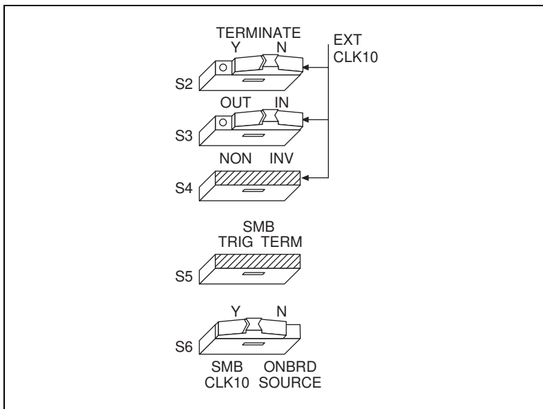
Figure C-6. Receive External CLK SMB and Drive to the Backplane Underterminated
