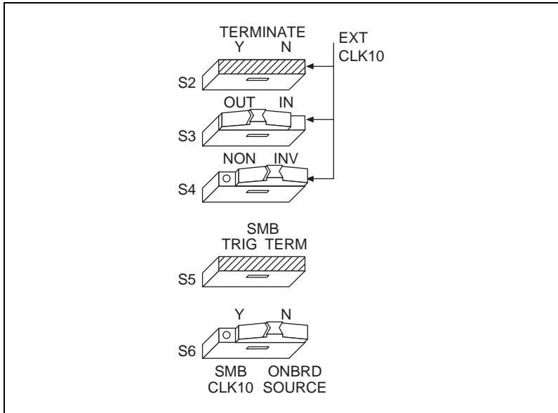
Figure C-8. Drive Inverted External CLK SMB
