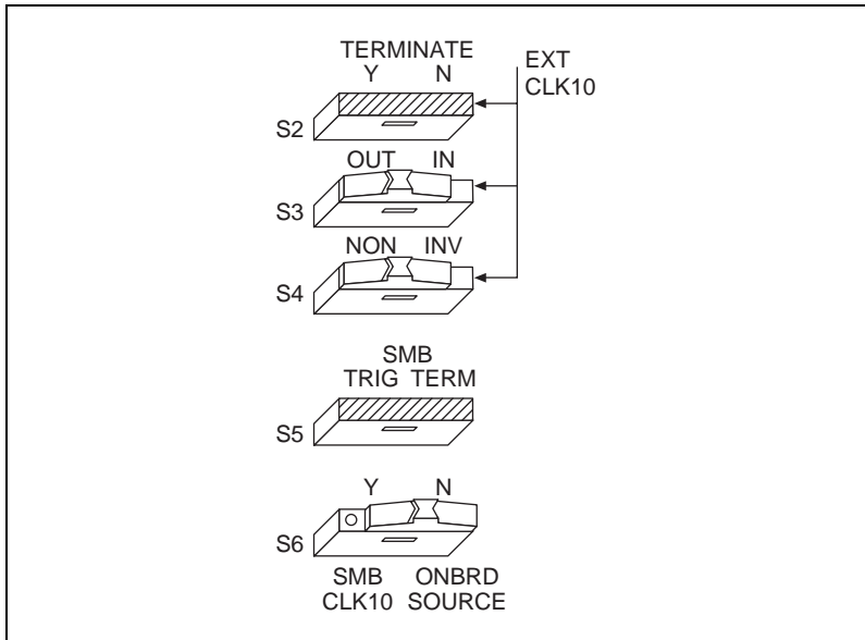
Figure C-9. Drive Non-Inverted External CLK SMB
