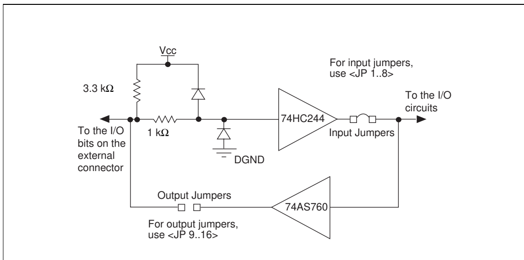
Figure 4-4. I/O Port Input and Output Hardware Circuitry
