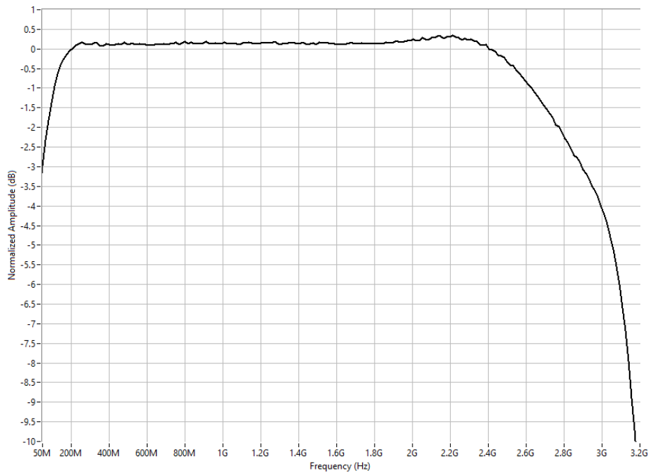
Figure 11. Analog Output Single Channel Mode Frequency Response, No Anti-Image Filter, Measured [21]
