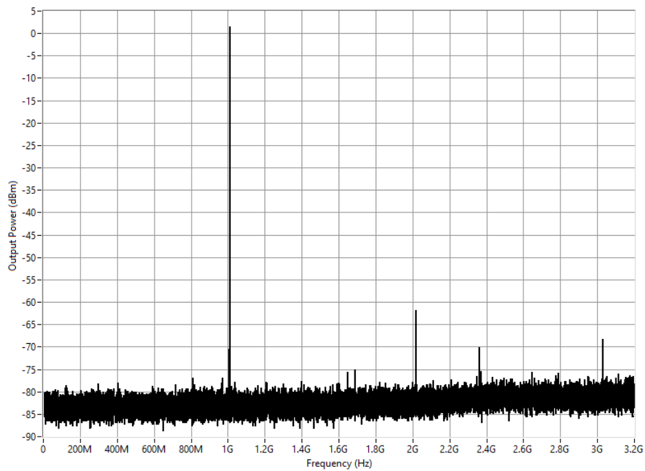
Figure 8. Single Tone Spectrum (Dual Channel Mode, 1.01 GHz 0 dBFS), Measured [19]
