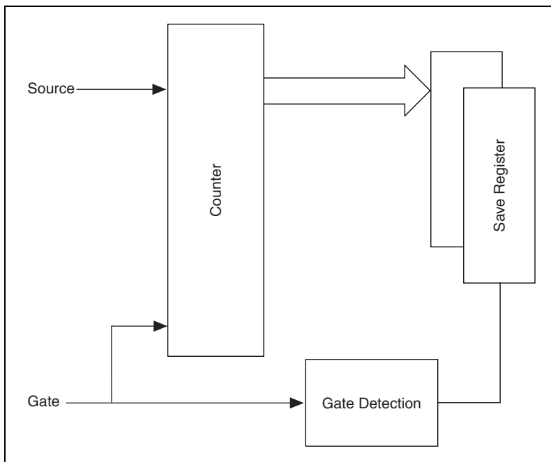
Figure 1-4. Measurement Data Flow
