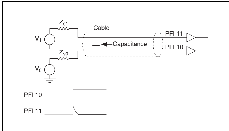
Figure 3-10. Crosstalk Example
