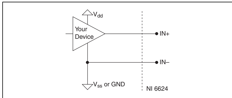
Figure 3-4. Connecting as Referenced to Ground
