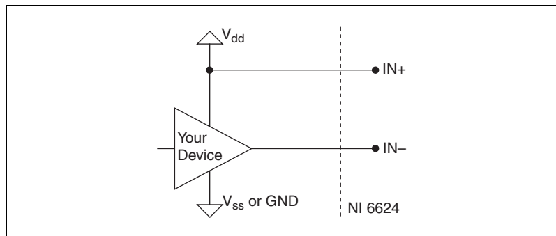
Figure 3-5. Connecting as Referenced to the Supply
