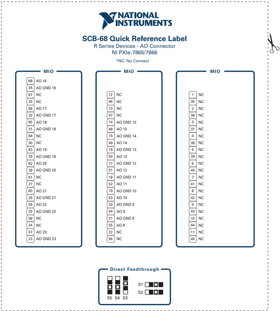
Figure 4. AO Connector for NI PXIe-7865/7866
