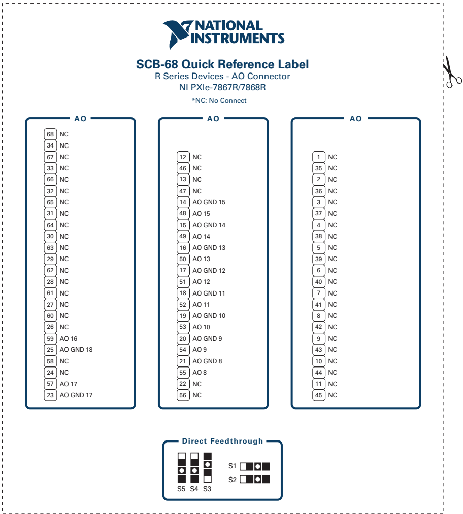
Figure 6. AO Connector for NI PXIe-7867R/7868R
