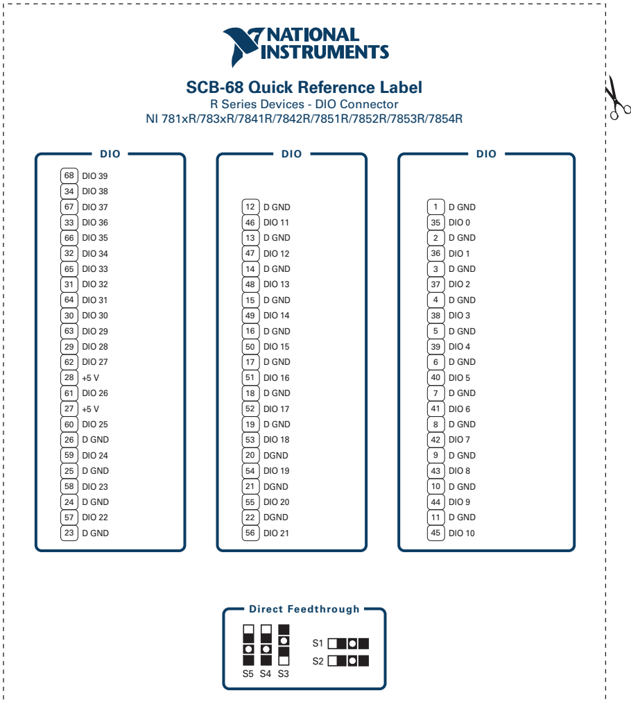
Figure 9. DIO Connector for NI 781xR/783xR/7841R/7842R/7851R/7852R/7853R/7854R
