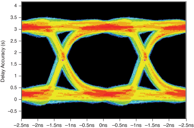
Figure 3. Characteristic Eye Diagram (High Impedance)
