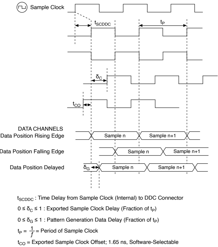
Figure 7. Generation Timing Diagram
