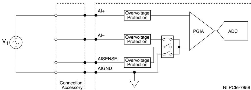
Figure 2. Connecting Referenced Single-Ended Signals to the PCIe-7858
