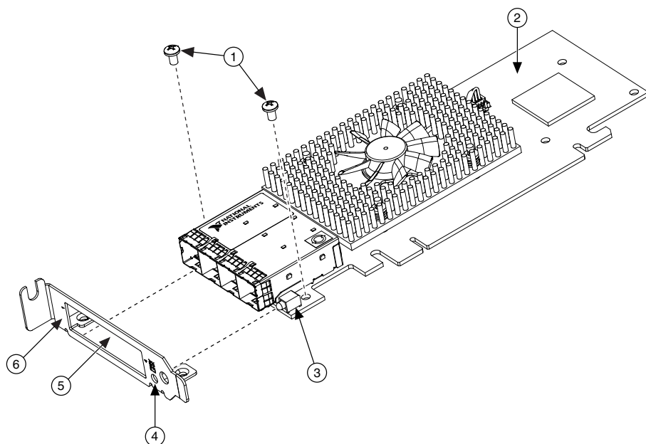
Figure 10. Removing the Standard Bracket from the PCIe-8398
