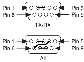
Figure 6. RS-232 Loopback
