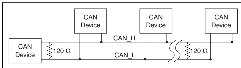
Figure B-5. Termination Resistor Placement
