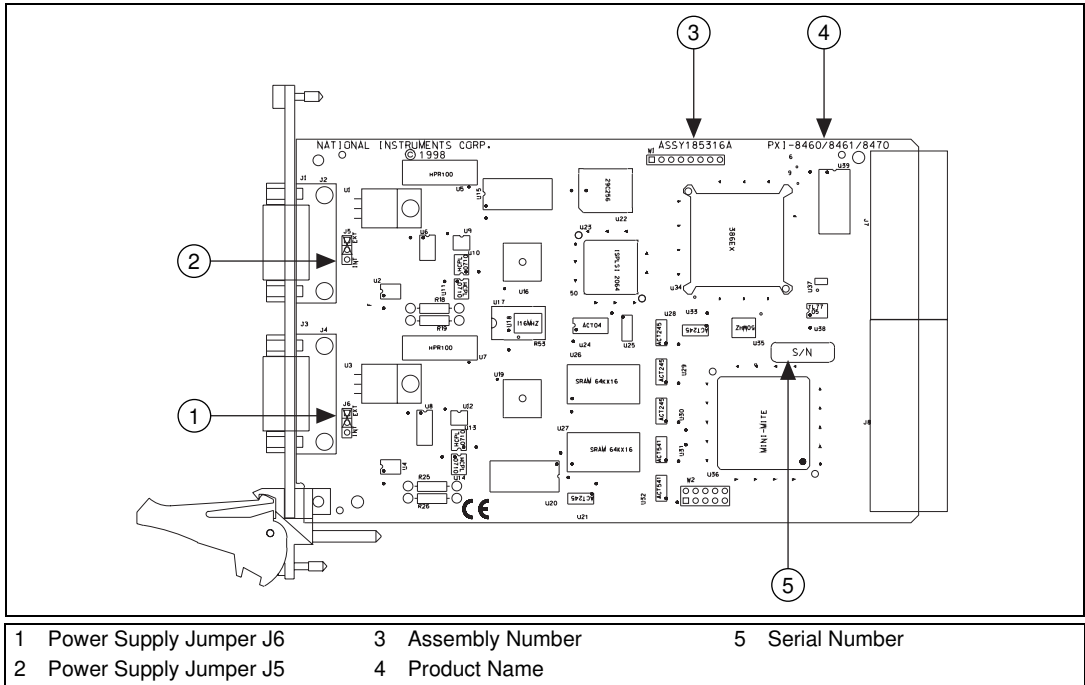
Figure B-3. PXI-8461 Part Locator Diagram
