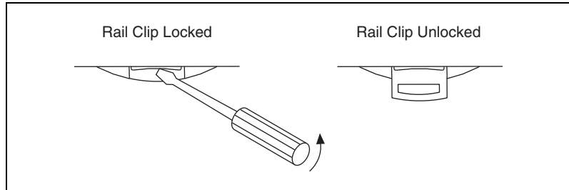
Figure 2-10. DIN Rail Clip
