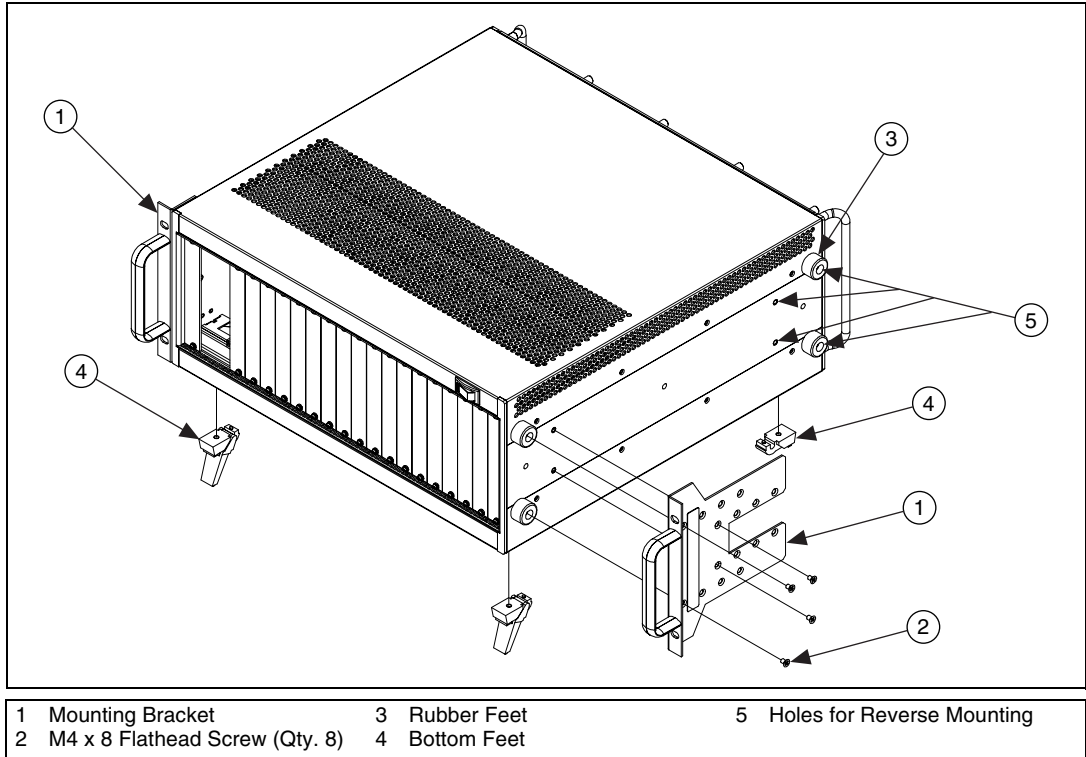
Figure 1. PXI-1006 in Rack Mount Configuration
