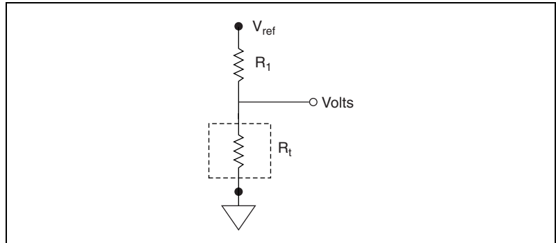
Figure 5-2. Circuit Diagram of a Thermistor in a Voltage Divider
