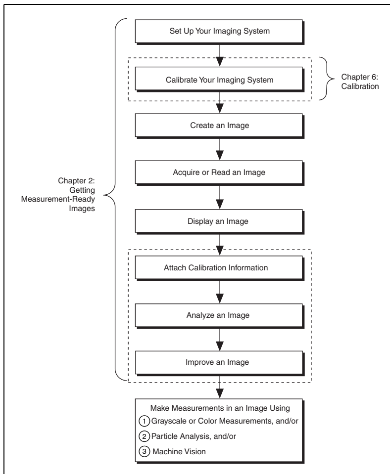
Figure 1-1. General Steps to Designing a Vision Application
