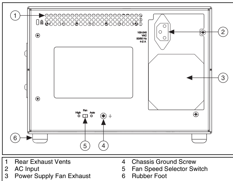
Figure 1-2. Rear View of the PXI-1031 Chassis
