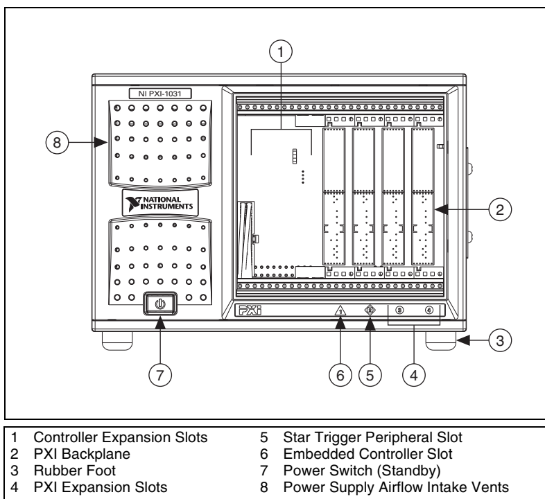
Figure 1-1. Front View of the PXI-1031 Chassis
