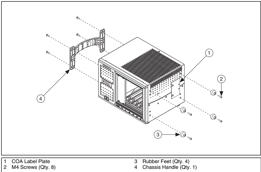
Figure 1. 4–6 Slot PXI Chassis with Optional Handle/Foot Kit
