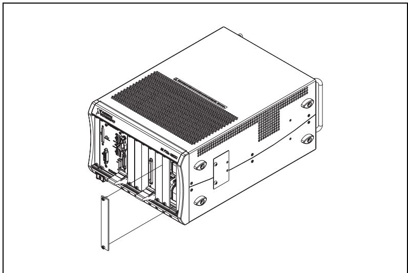
Figure 2. Installing a PXI filler panel
