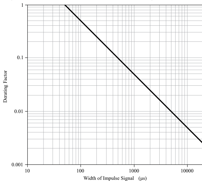
Figure 6. Maximum Cycle Rate Derating Factor by Pulse Width
