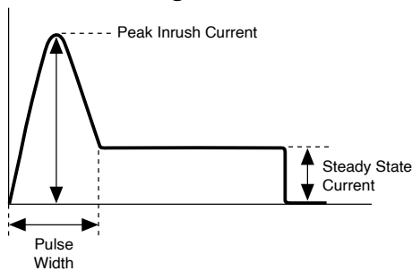
Figure 3. Switching Current Waveform
