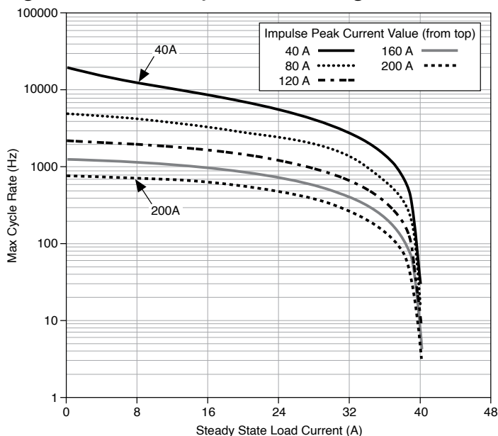
Figure 4. Maximum Cycle Rate for Single Path Closed
