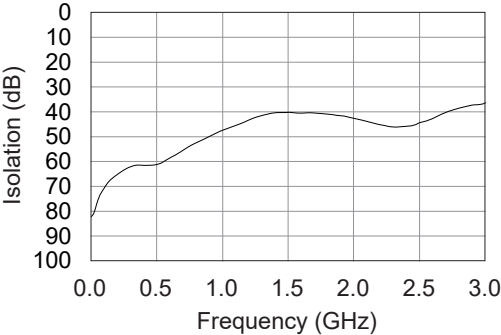
Figure 3. Typical Isolation
