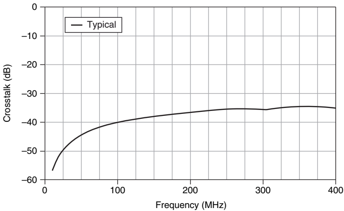
Figure 7. Typical Crosstalk
