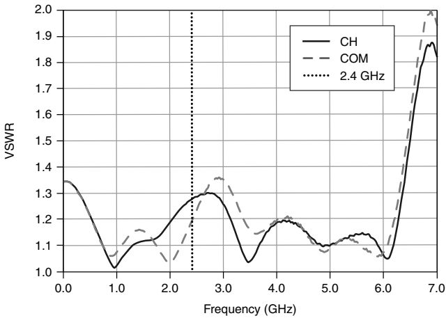
Figure 2. Typical VSWR
