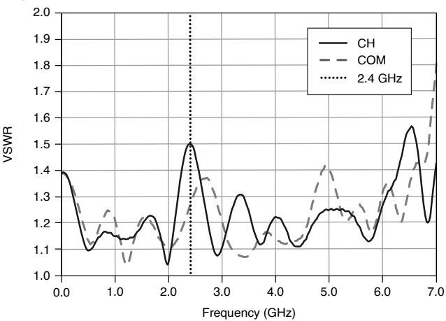
Figure 2. Typical VSWR
