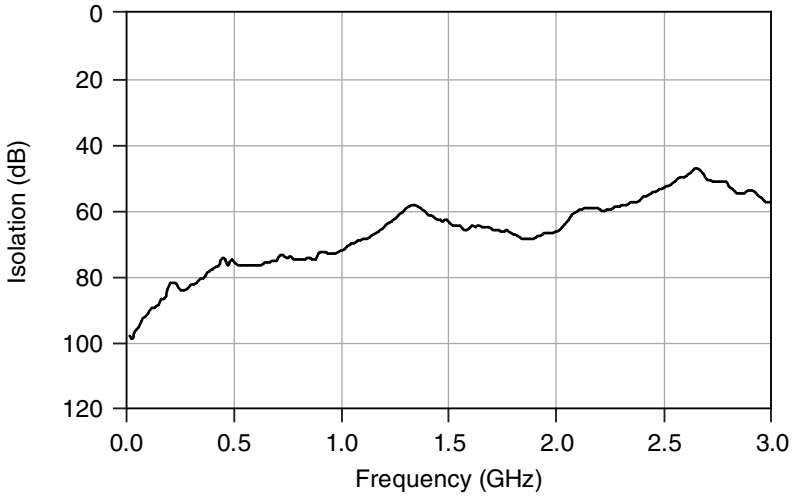
Figure 4. Isolation, Typical
