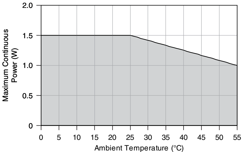
Figure 5. Termination Derating
